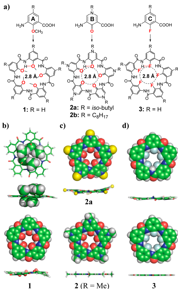
Figure 1. Structural features of pentamers 1–3. (a) Structures of pentamers 1–3 derived from monomeric building blocks A–C, respectively, each containing an interior cavity of \sim 2.8 \text{ \AA} in diameter defined by oxygen or fluorine atoms. (b–d) The top and side views of crystal structures 1 , 2a and its computationally determined structure as well as 3 and its computationally determined structure. In the bottom of (b), the five interior methyl groups were removed for an unblocked view of a sizable cavity in 1 . The yellow balls in (c) refer to the five exteriorly arrayed tert -butyl groups that have been removed for clarity of view. The computationally determined structures for both 2a and 3 illustrate five-fold symmetry and a planar pentagonal backbone contained in this family of pentamers.
