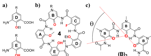
Figure 2. (a) Schematic illustration of additional building blocks D and E for constructing macrocyclic hybrid pentamers such as 4 (b). Amidated trimer as represented by (B) 3 in (c) was used for calculating \theta values and the number of residues ( n ) required for A–E to form a regular pentagon. In (c), angle \theta is defined by the atoms in red as the external angle of a pentagon to be formed, which will be computationally determined by the first principle calculation at the B3LYP/6-31G(d,p) level and compared to the crystallographically derived values.
